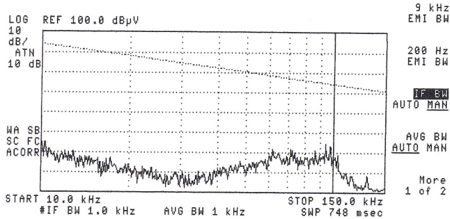
MIL-STD-361F scan w/ R/O SV28-12-20-1
